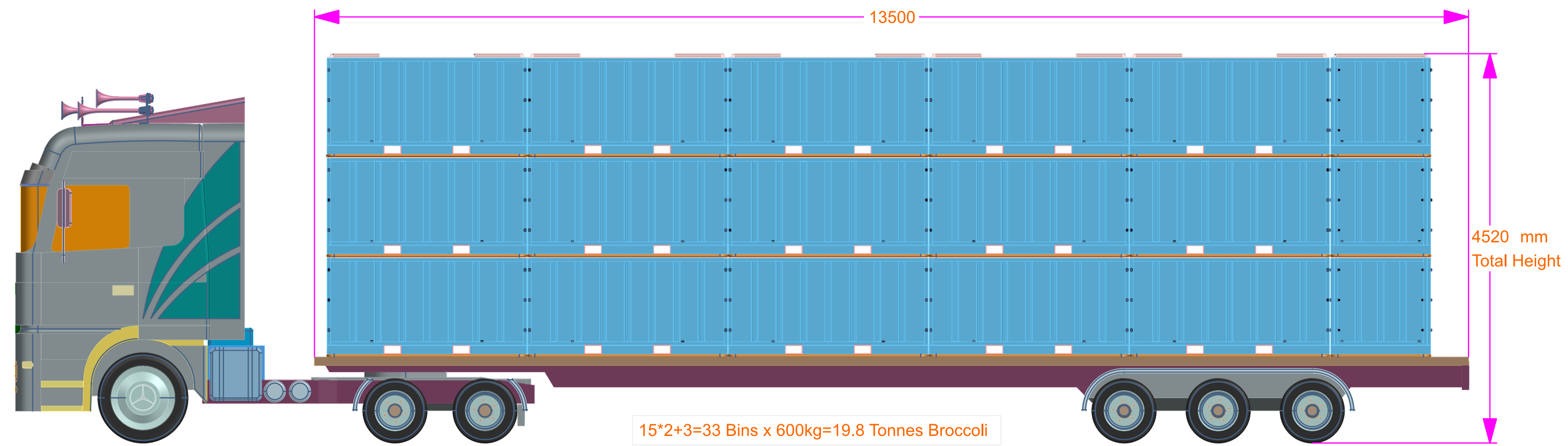
Side View
