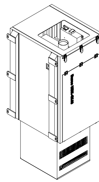
Isometric@20
