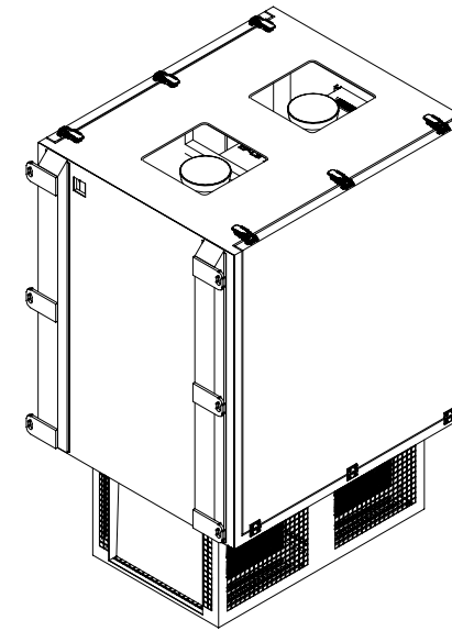
Isometric@6
