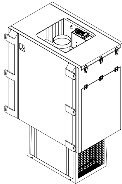
Isometric@15
