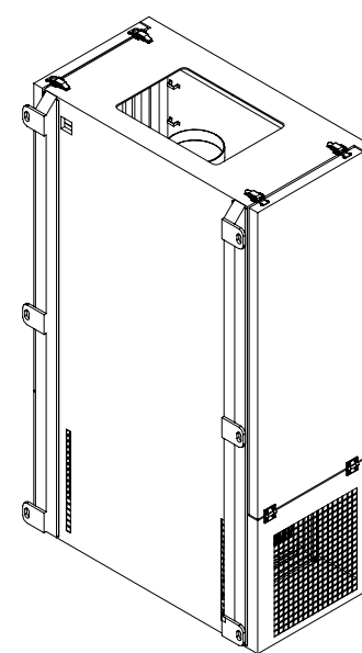
Isometric@11
